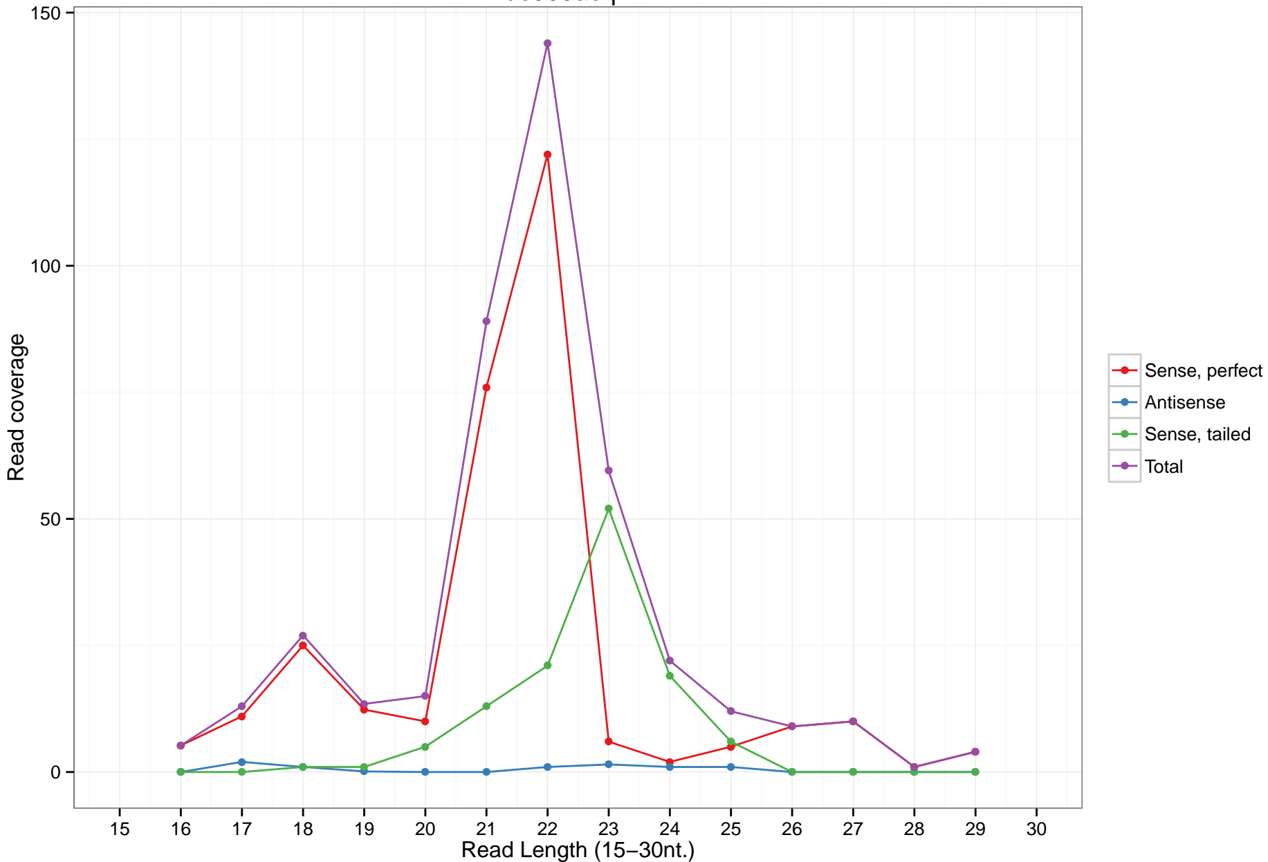
uc009acq.21
