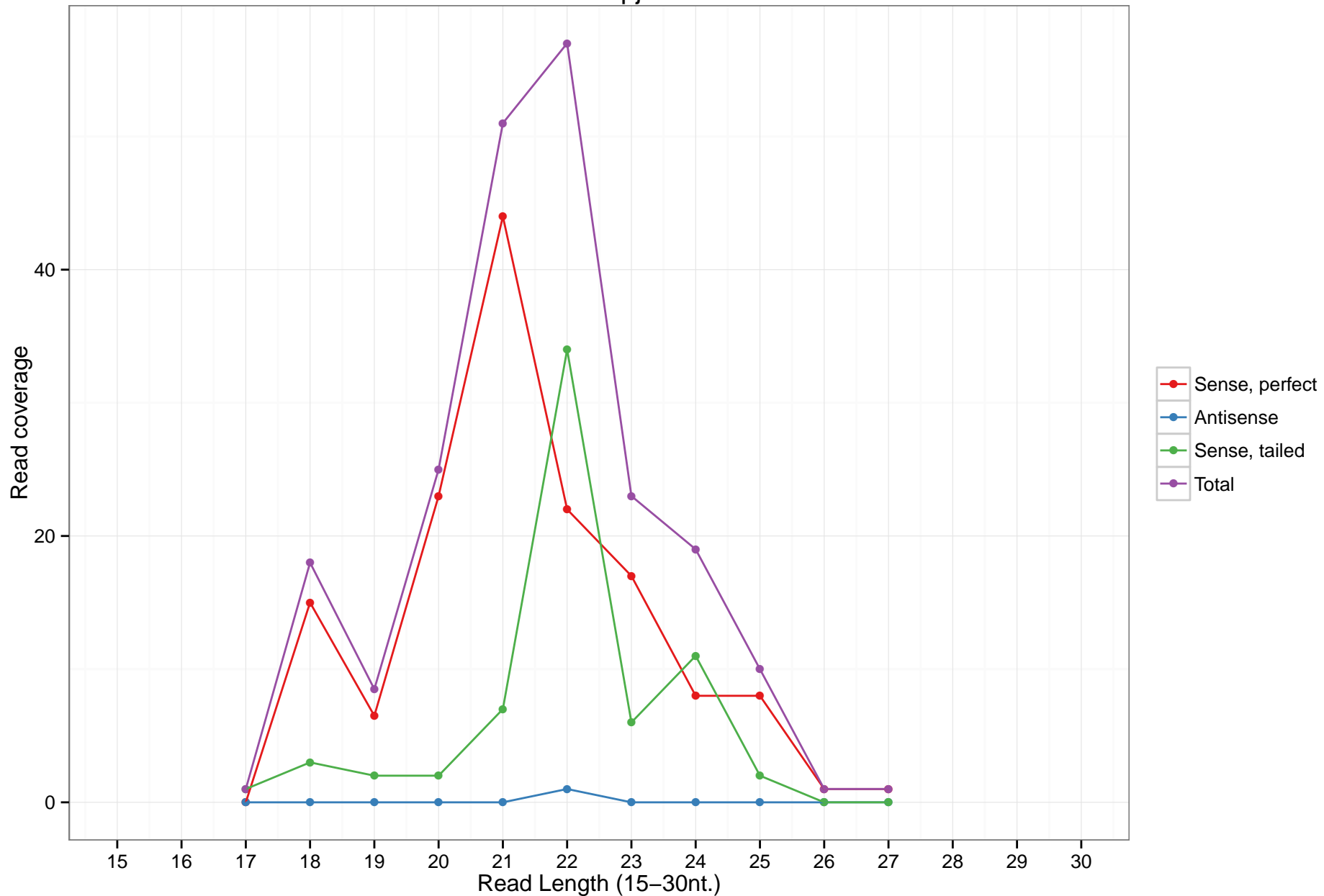
uc007kpj.2
