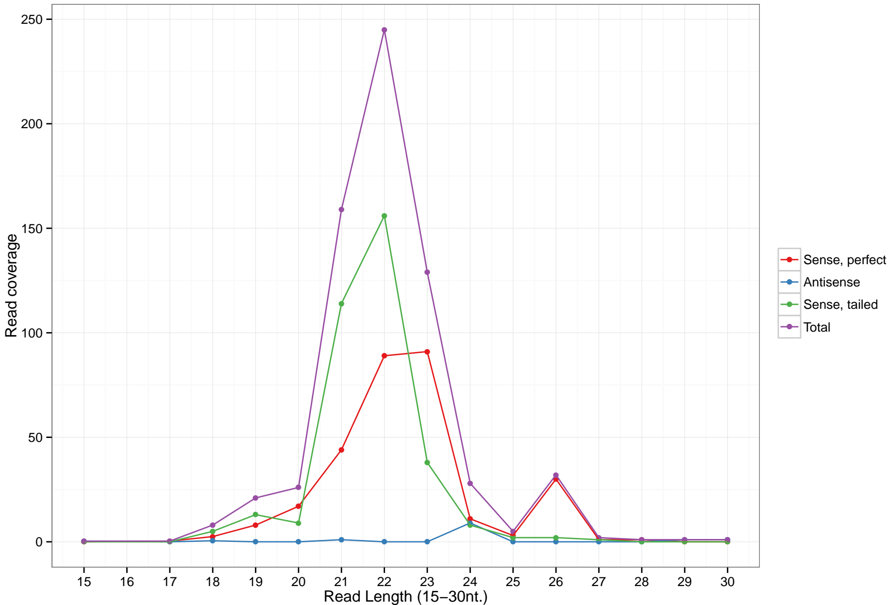
mmu-mir-6976
