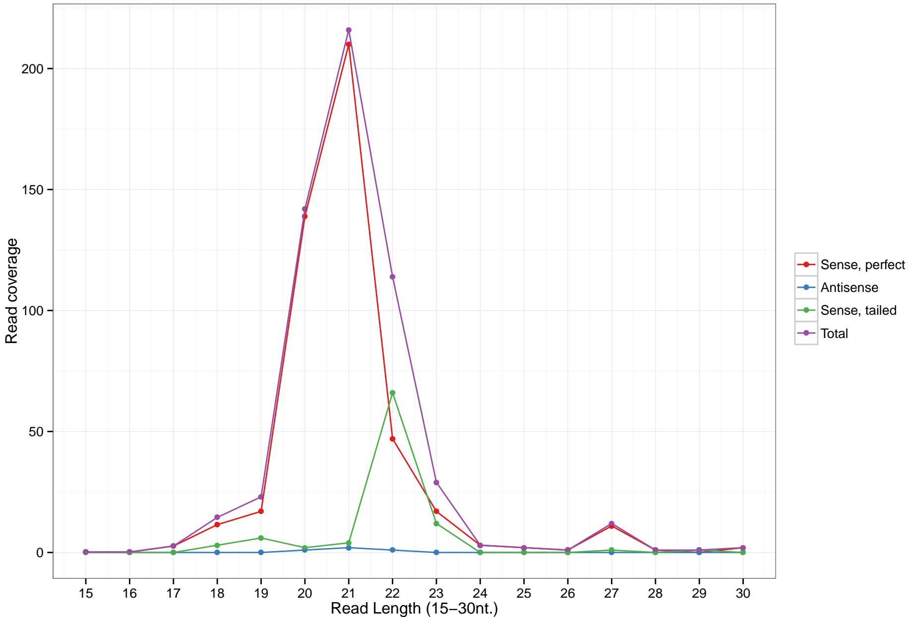
mmu-mir-6951
