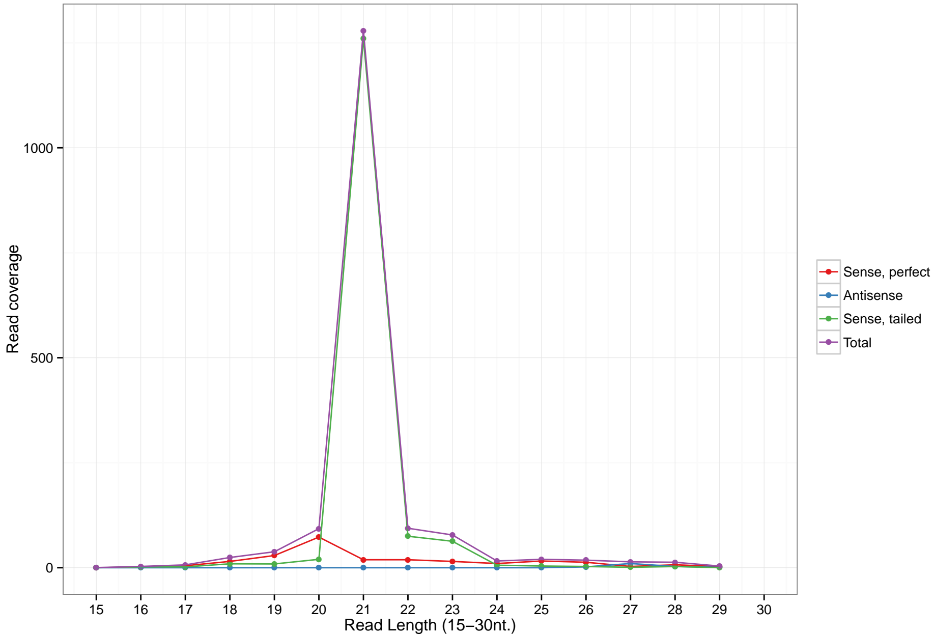
mmu-mir-6939
