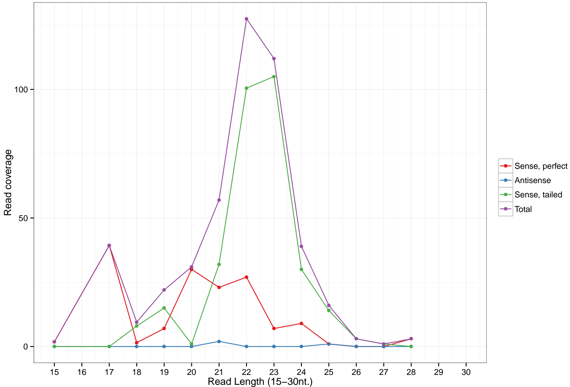
mmu-mir-6901
