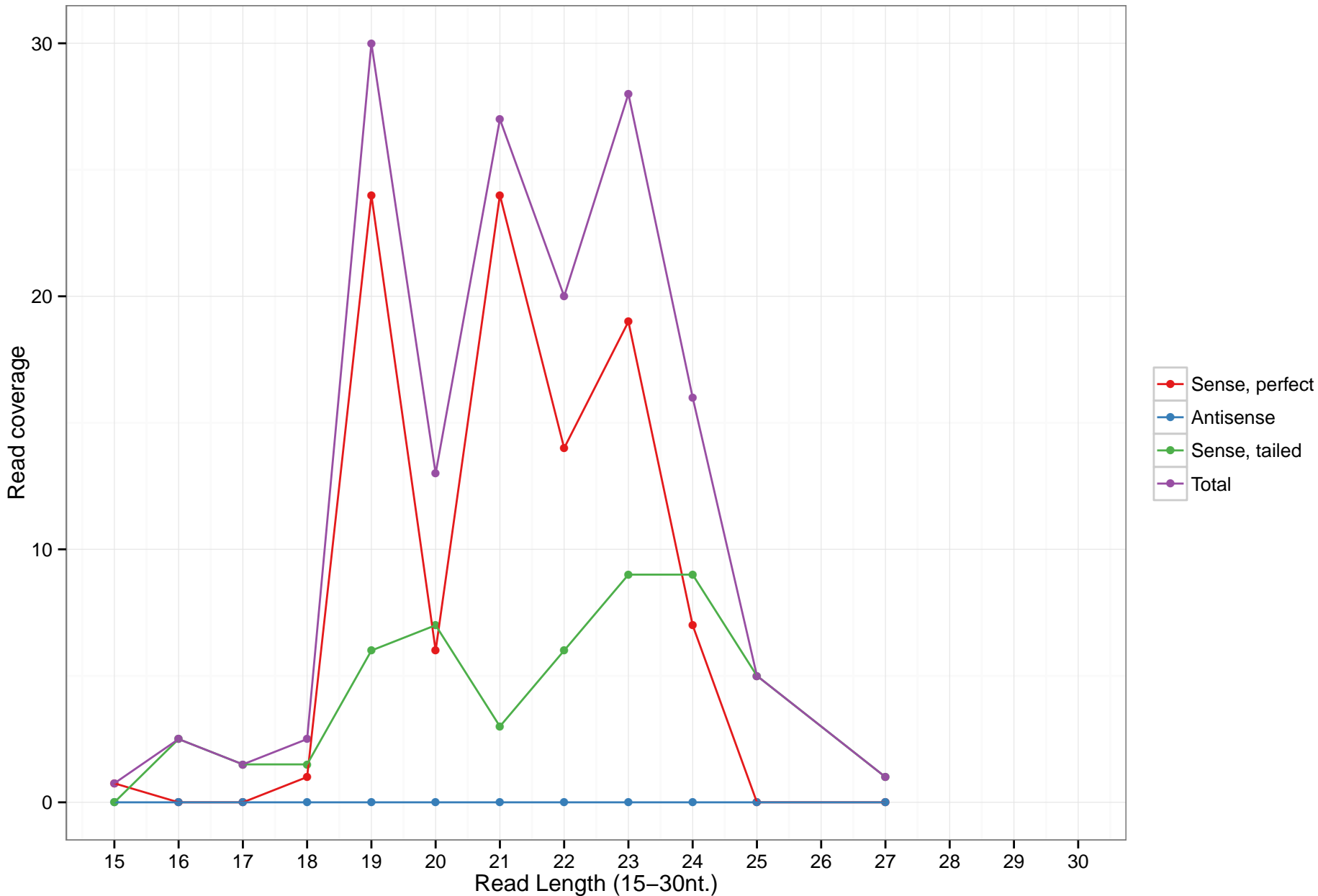
mmu-mir-1963
