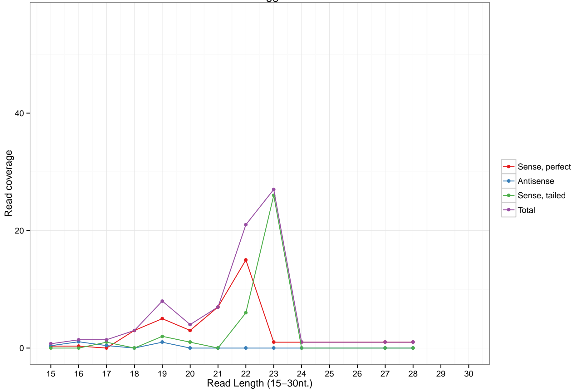
uc010fgg.2
