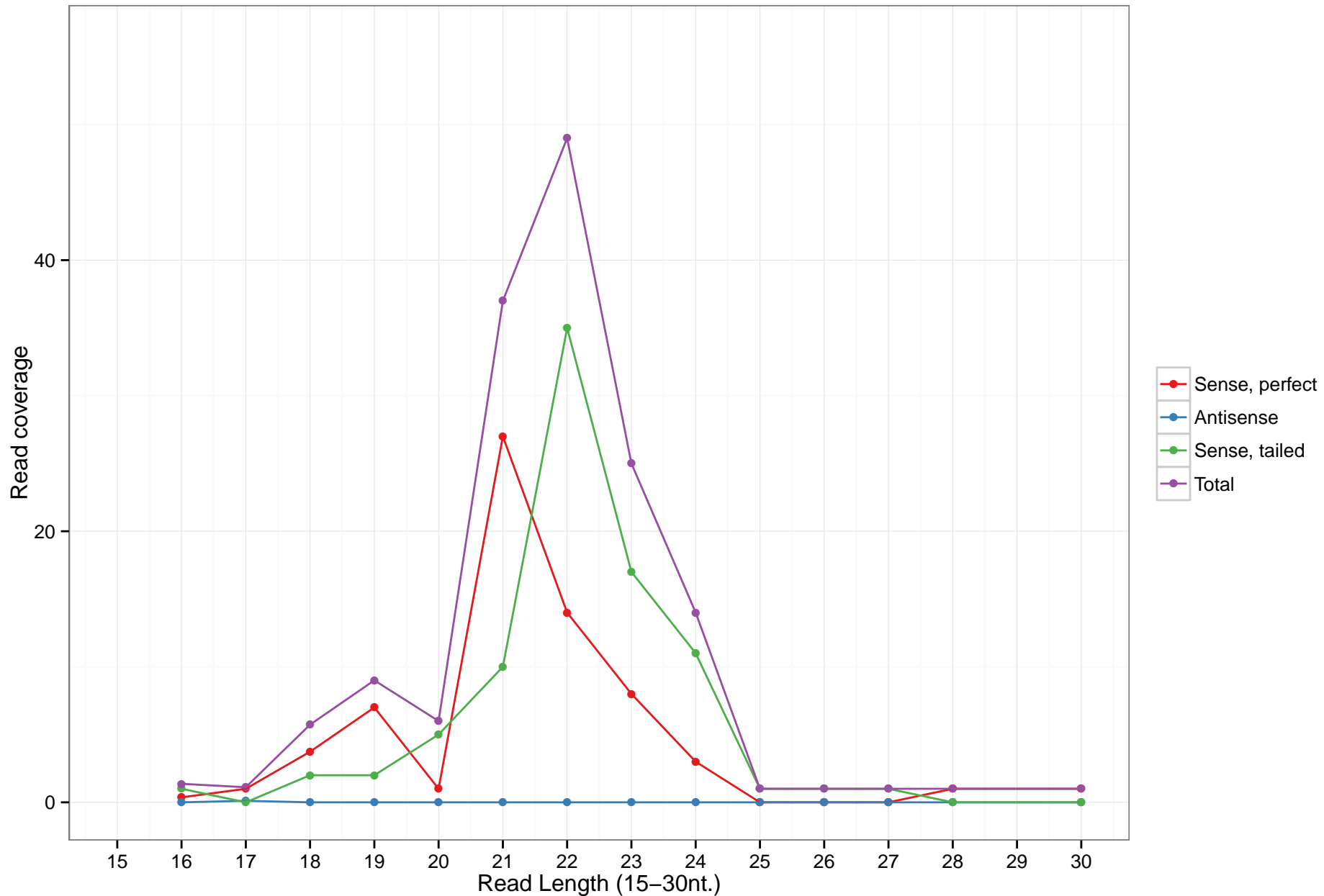
uc002owt.2
