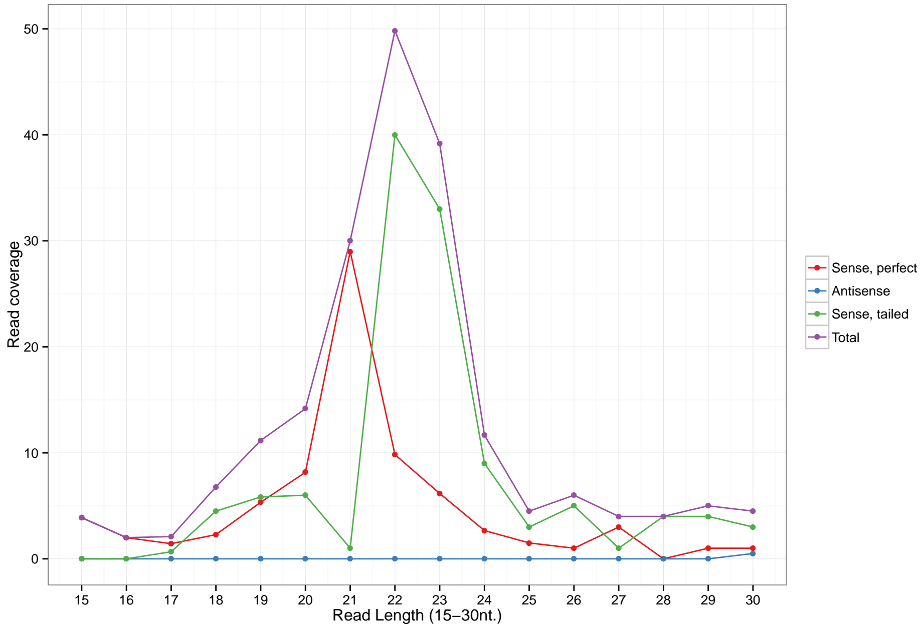
uc002ndi.2
