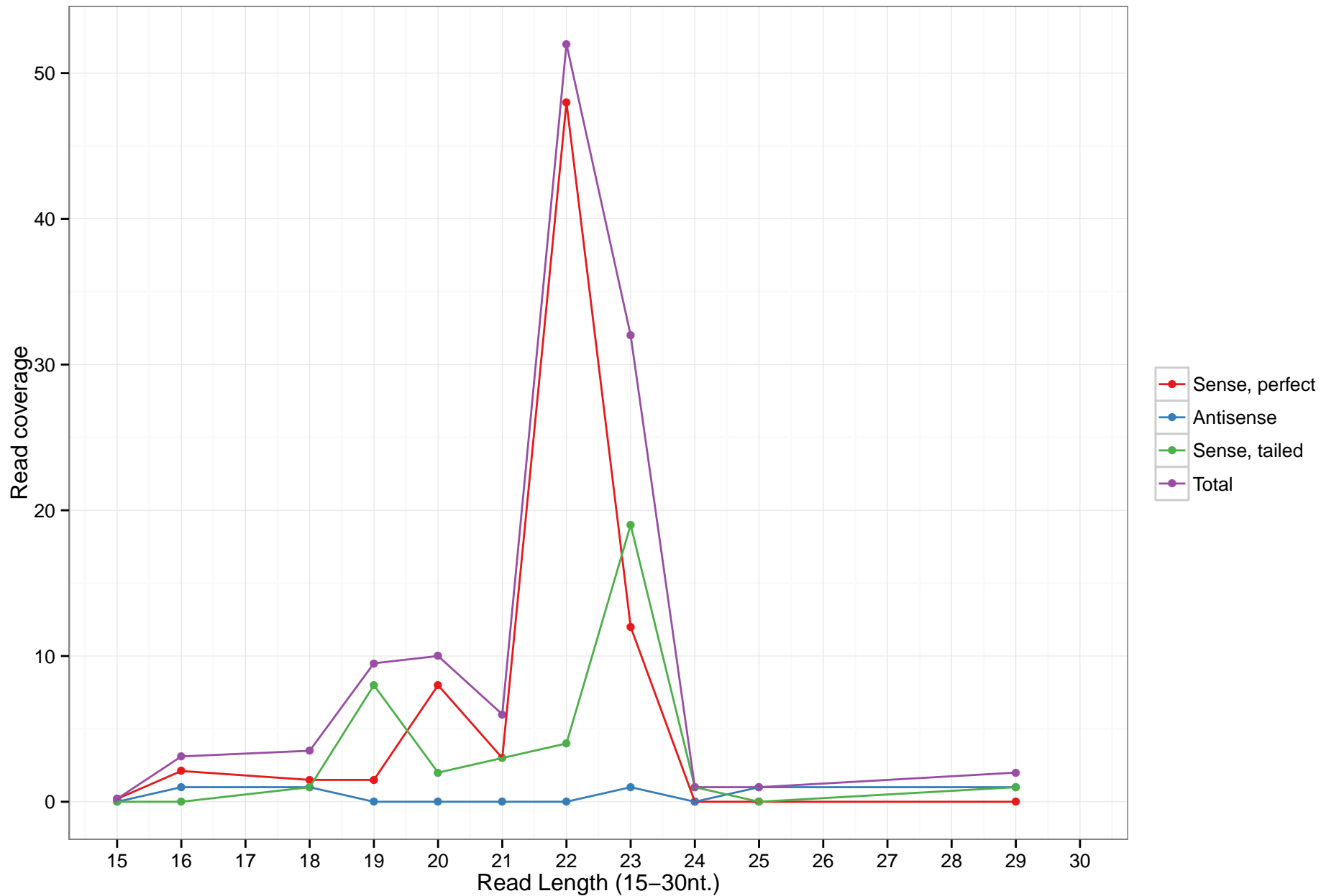
uc002mcx.7
