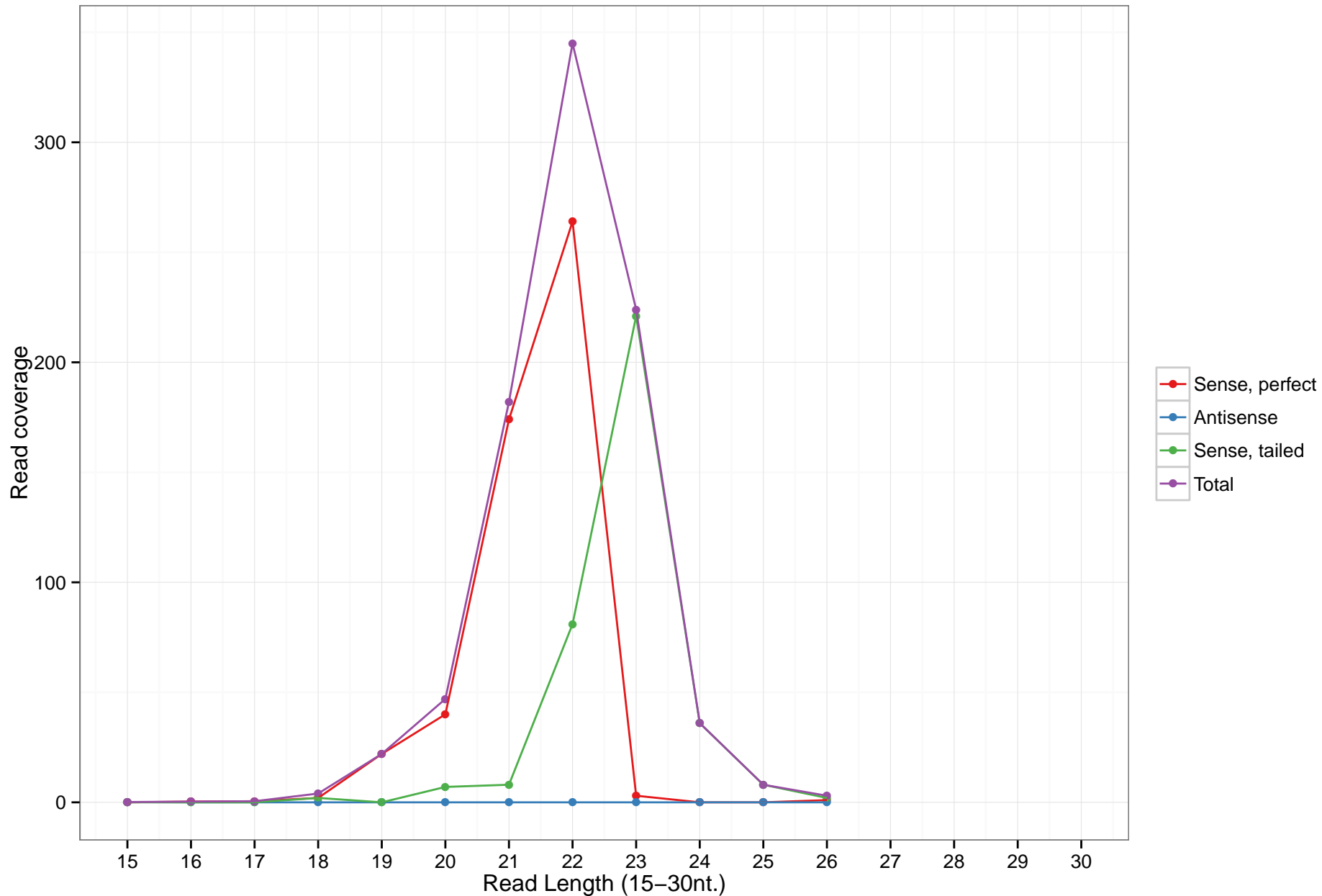
uc002fwx.16
