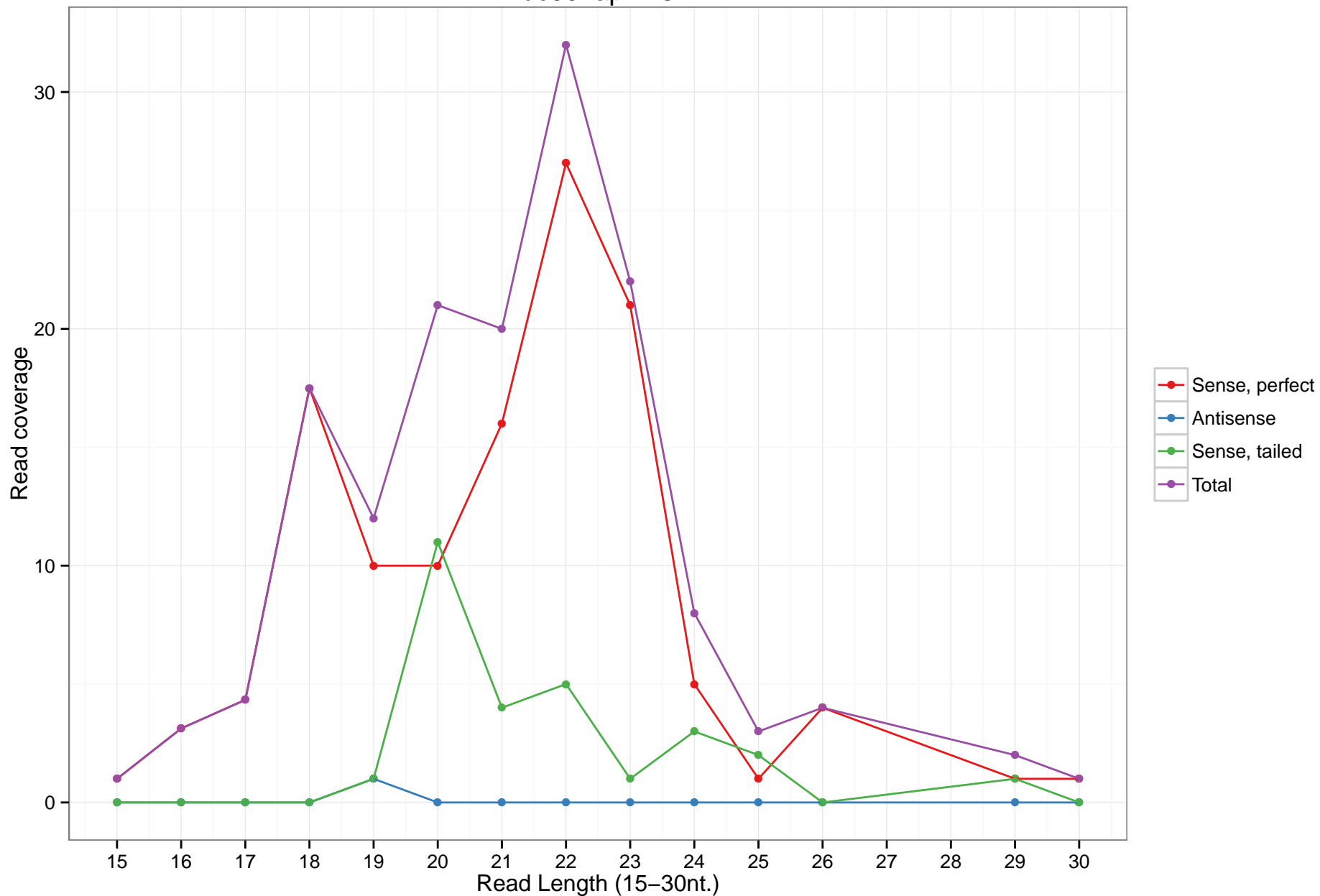
uc001api.1.6
