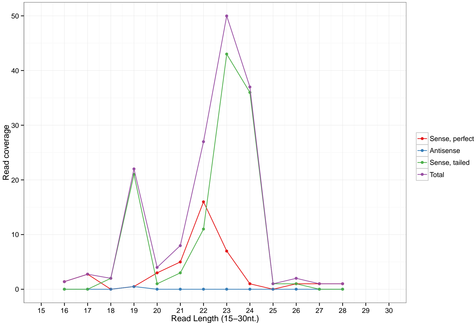
hsa-mir-7109
