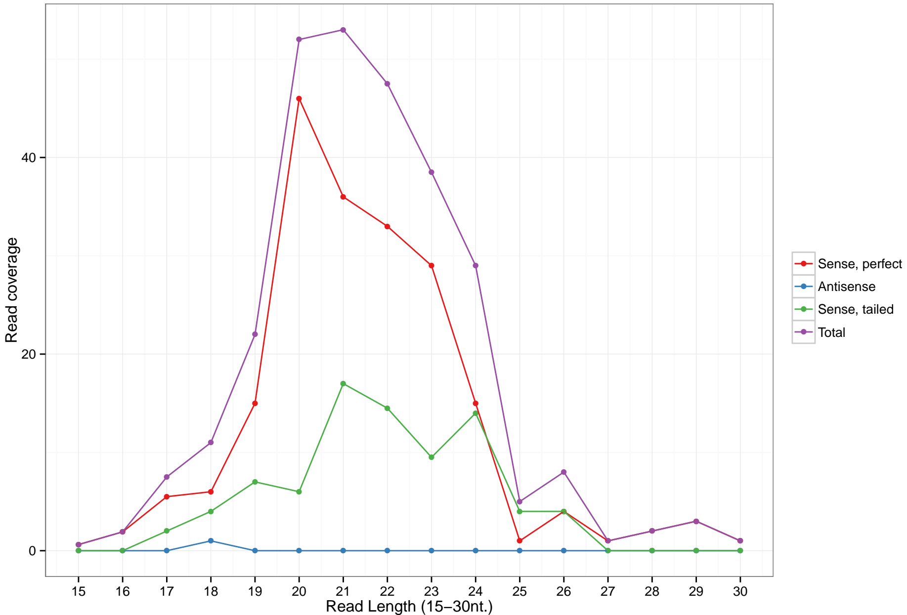
hsa-mir-6890
