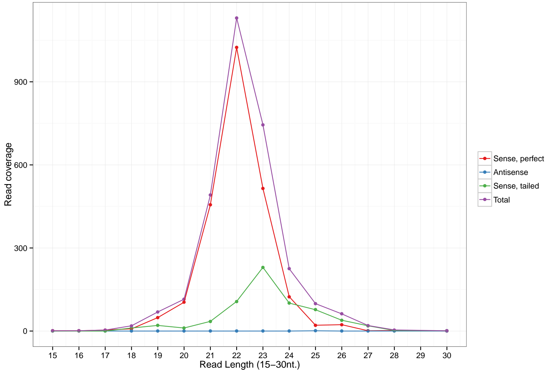
hsa-mir-6882
