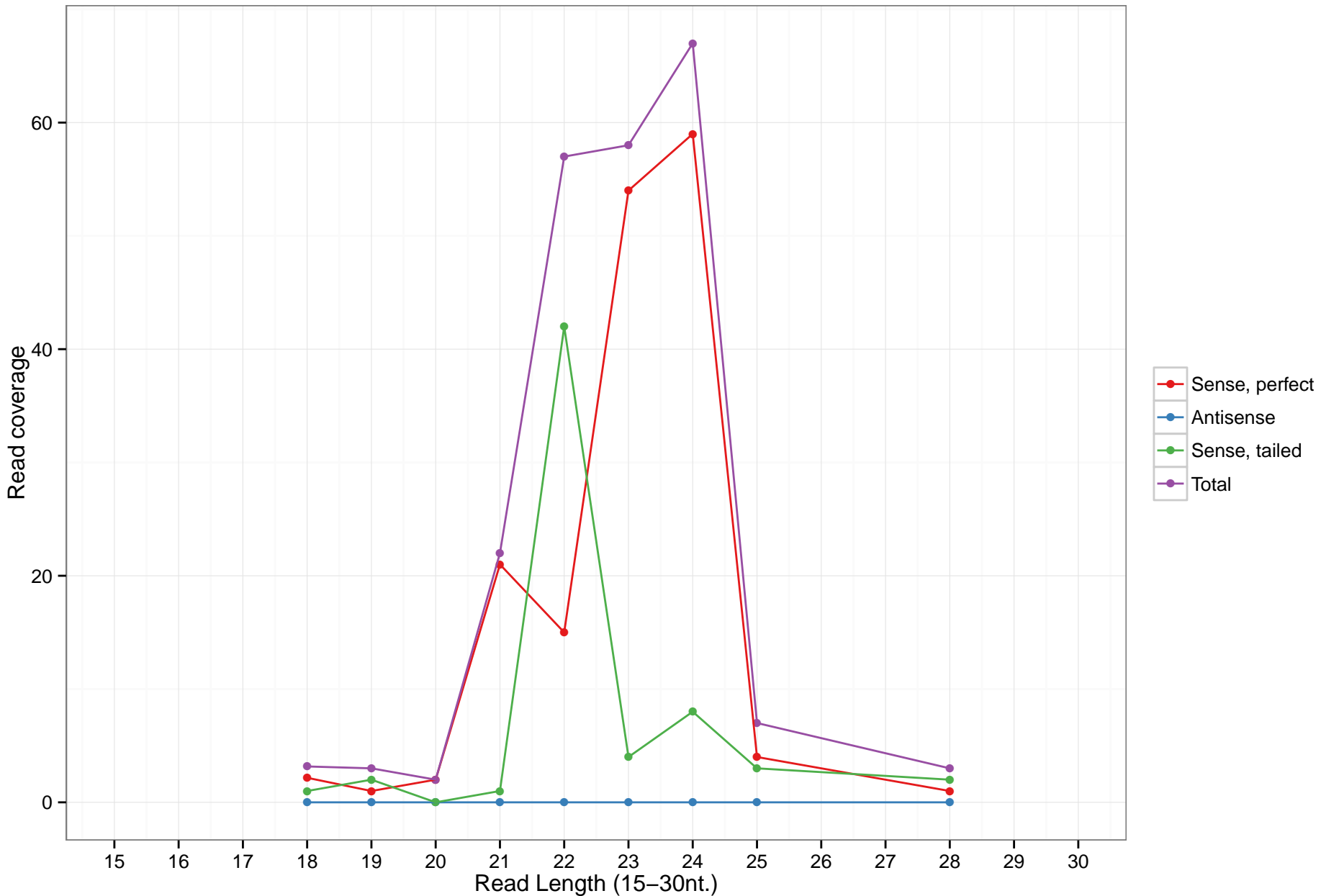
hsa-mir-6854
