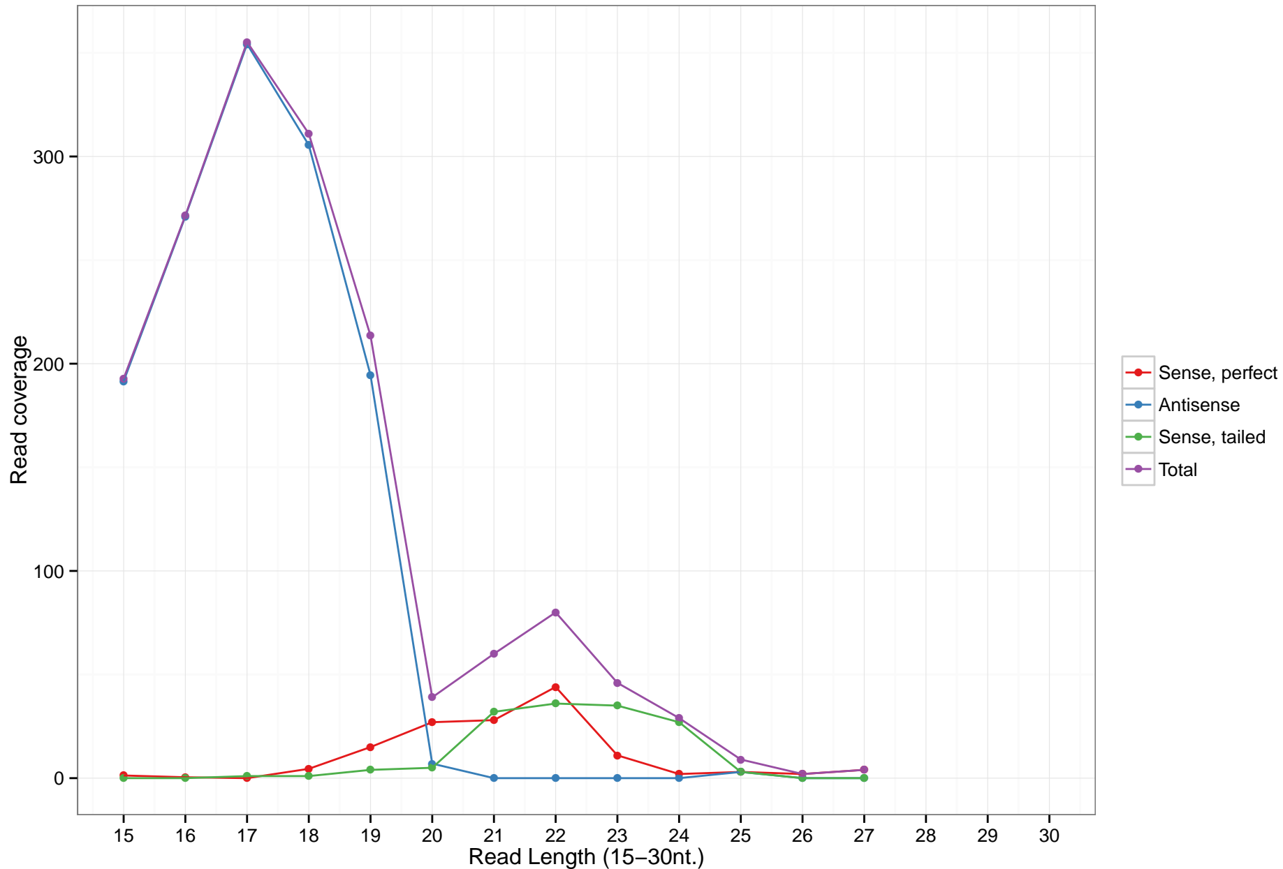
hsa-mir-6838
