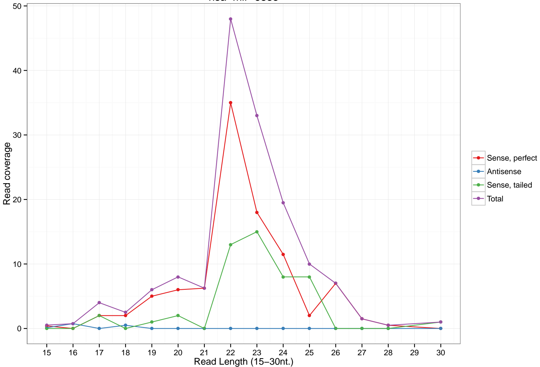
hsa-mir-6835
