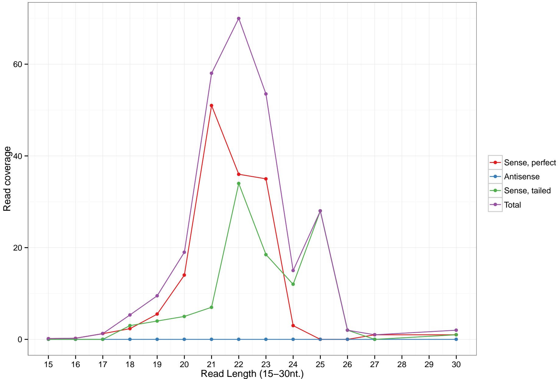
hsa-mir-6826
