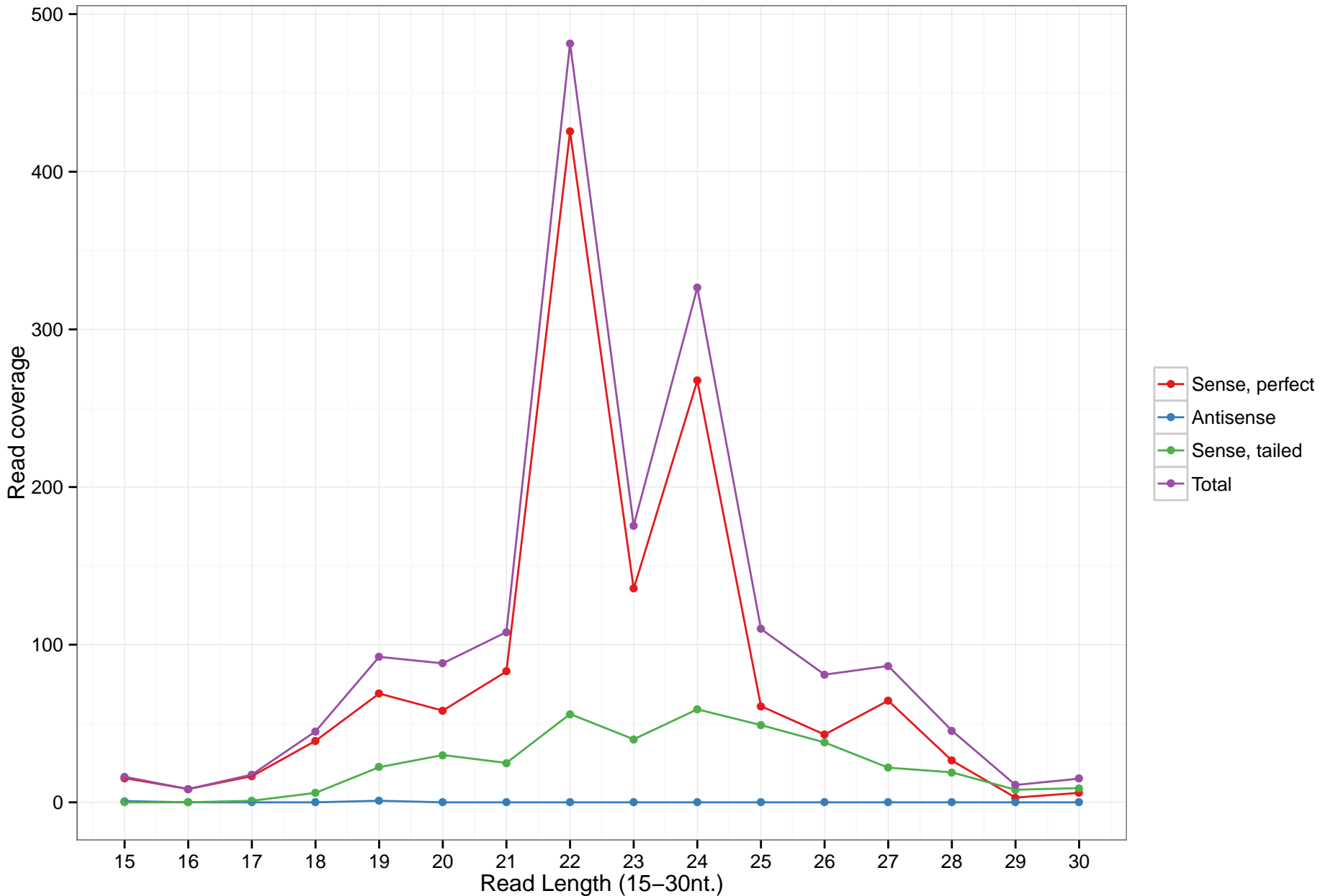
hsa-mir-6805
