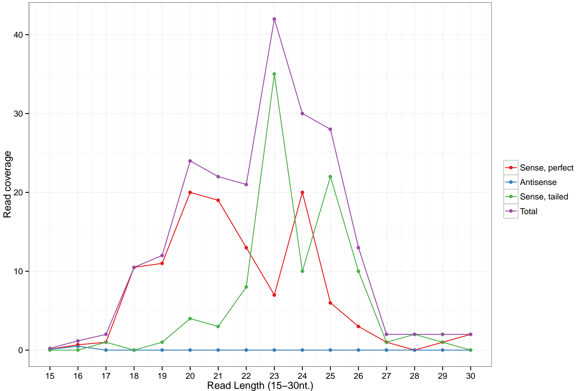
hsa-mir-6800
