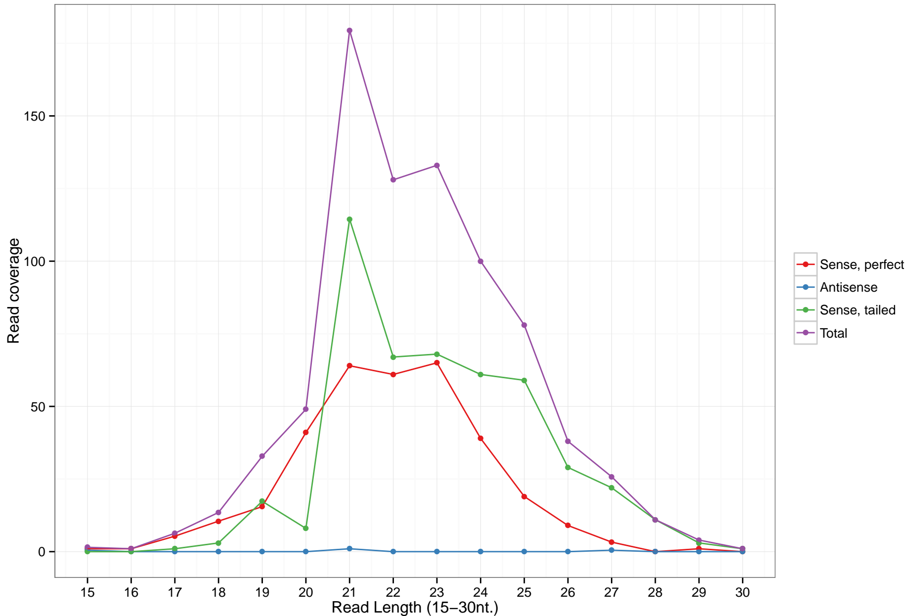
hsa-mir-6793
