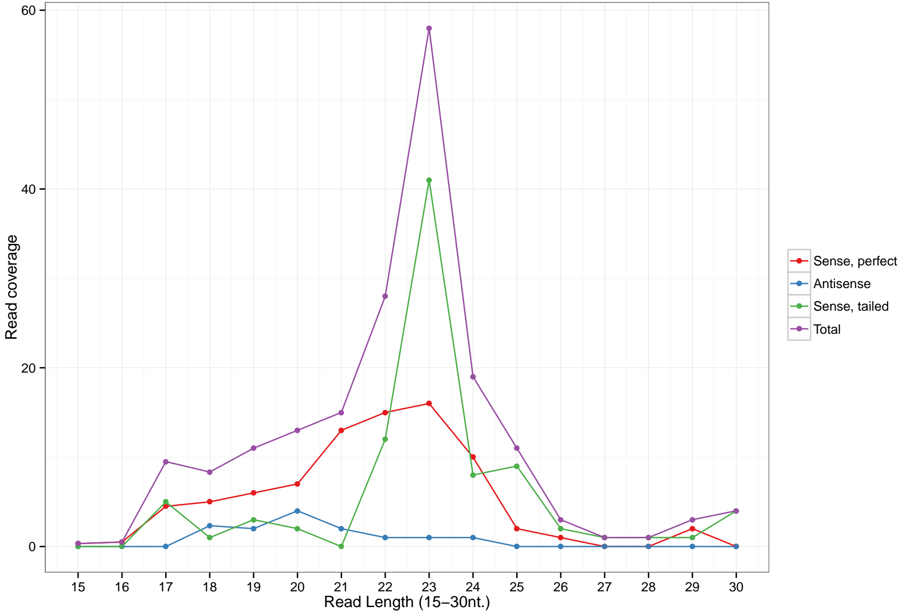
hsa-mir-6781
