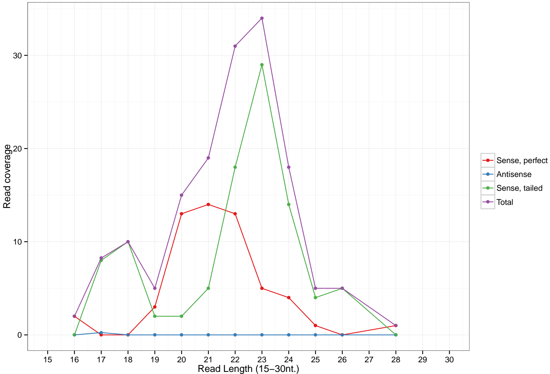
hsa-mir-6771
