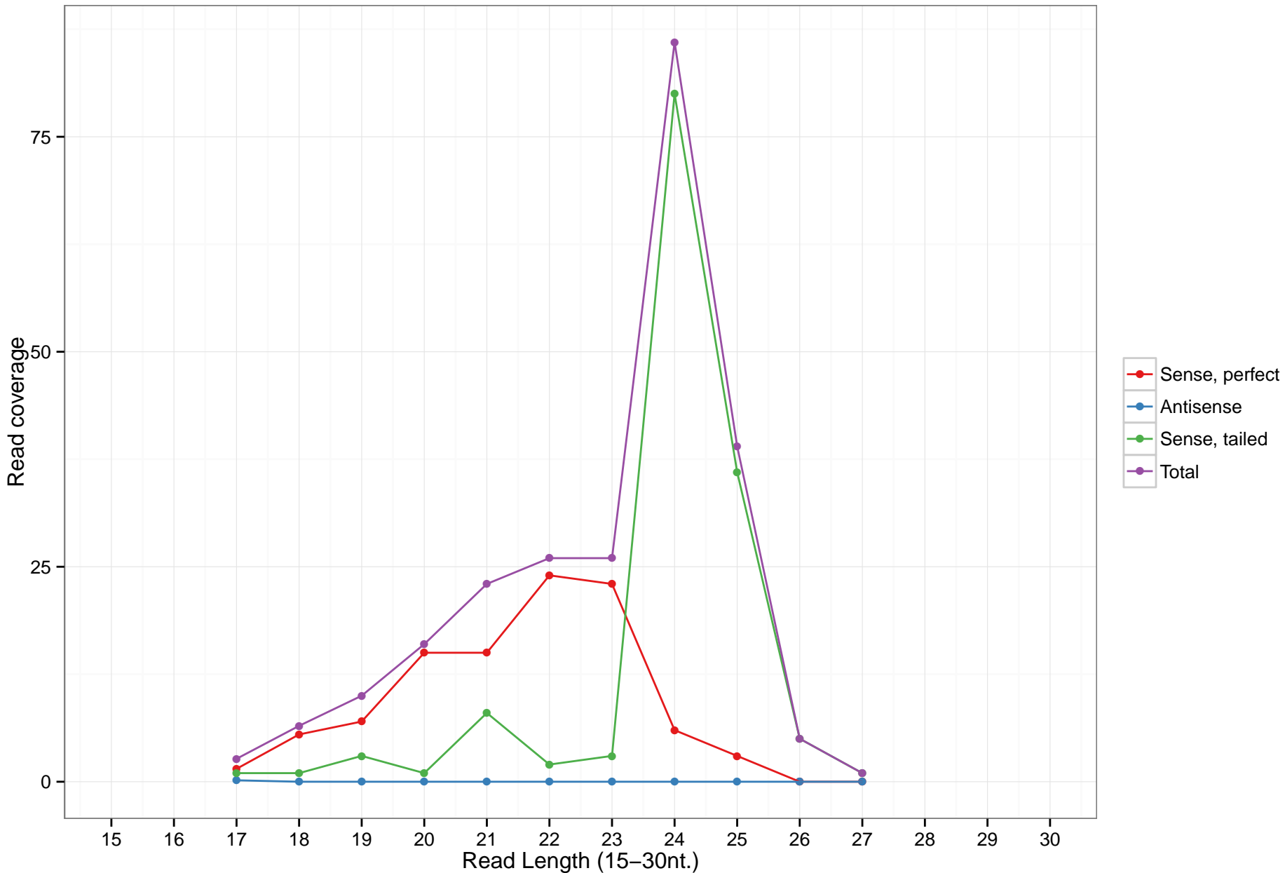
hsa-mir-6762
