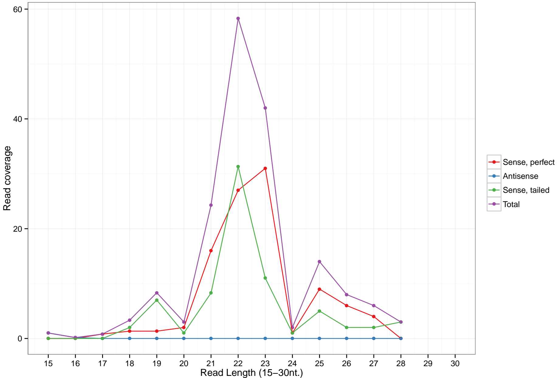
hsa-mir-6760
