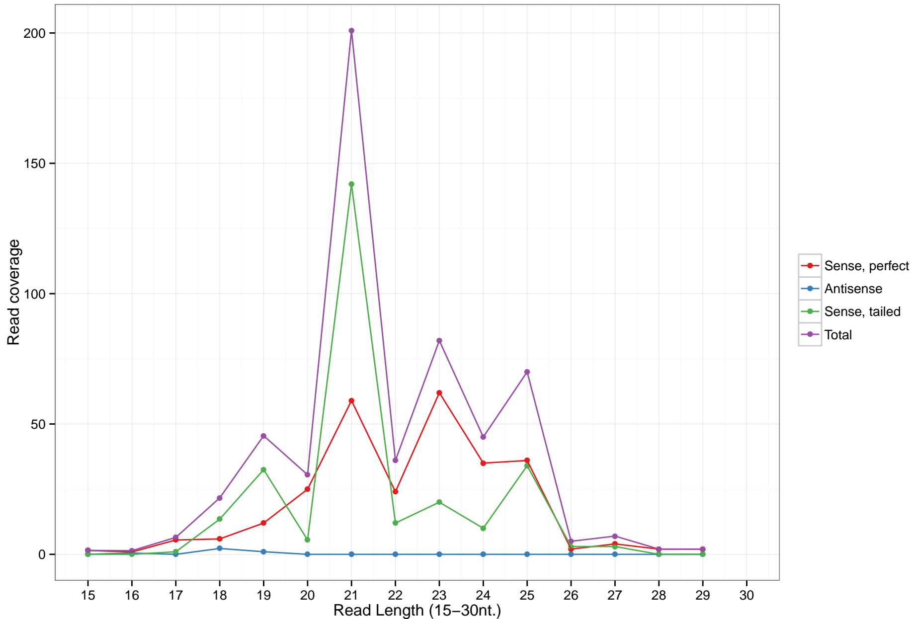
hsa-mir-6758
