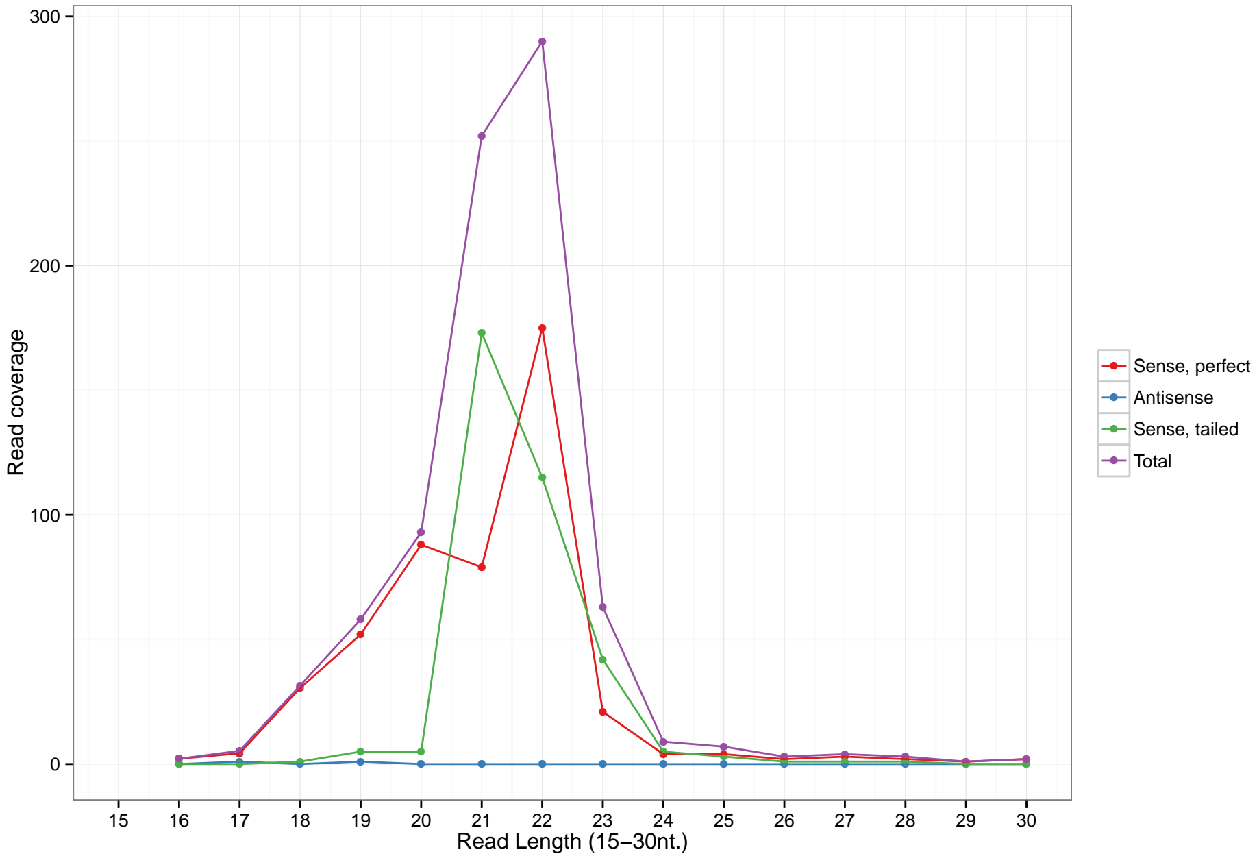
hsa-mir-6733
