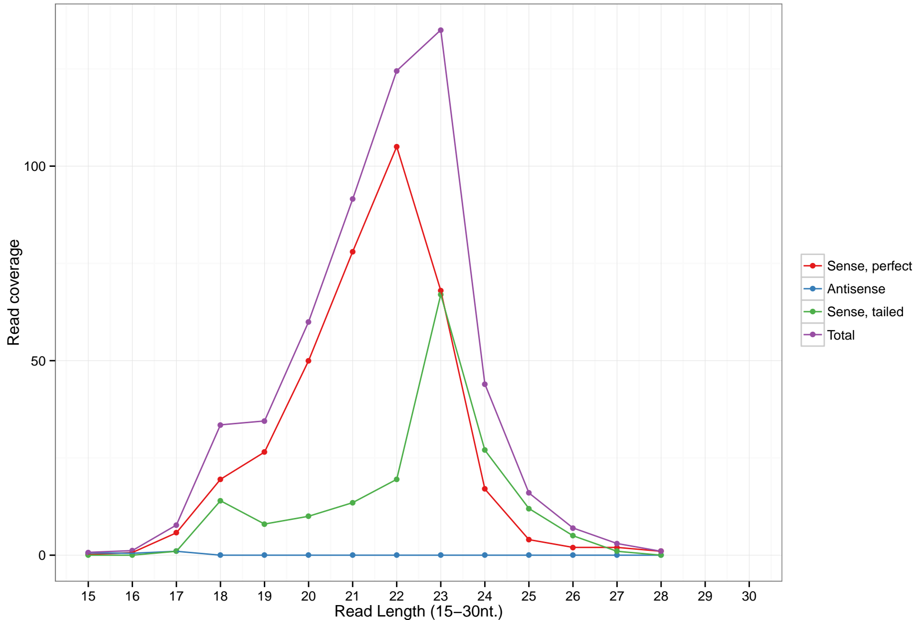
hsa-mir-6730
