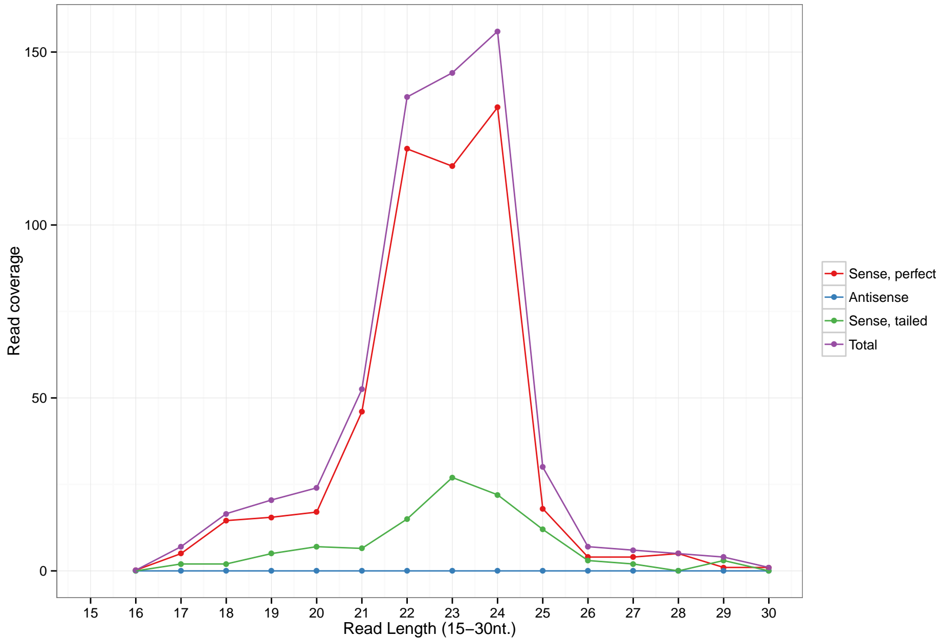
hsa-mir-5088
