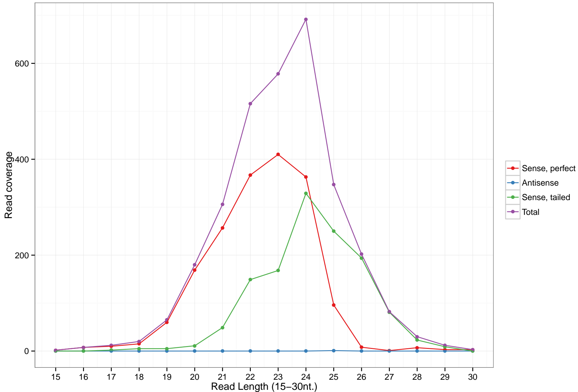
hsa-mir-4745
