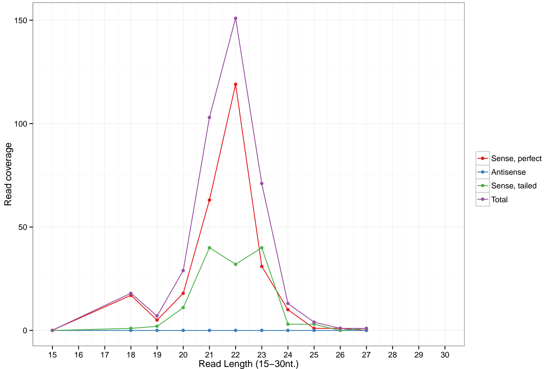
hsa-mir-4639
