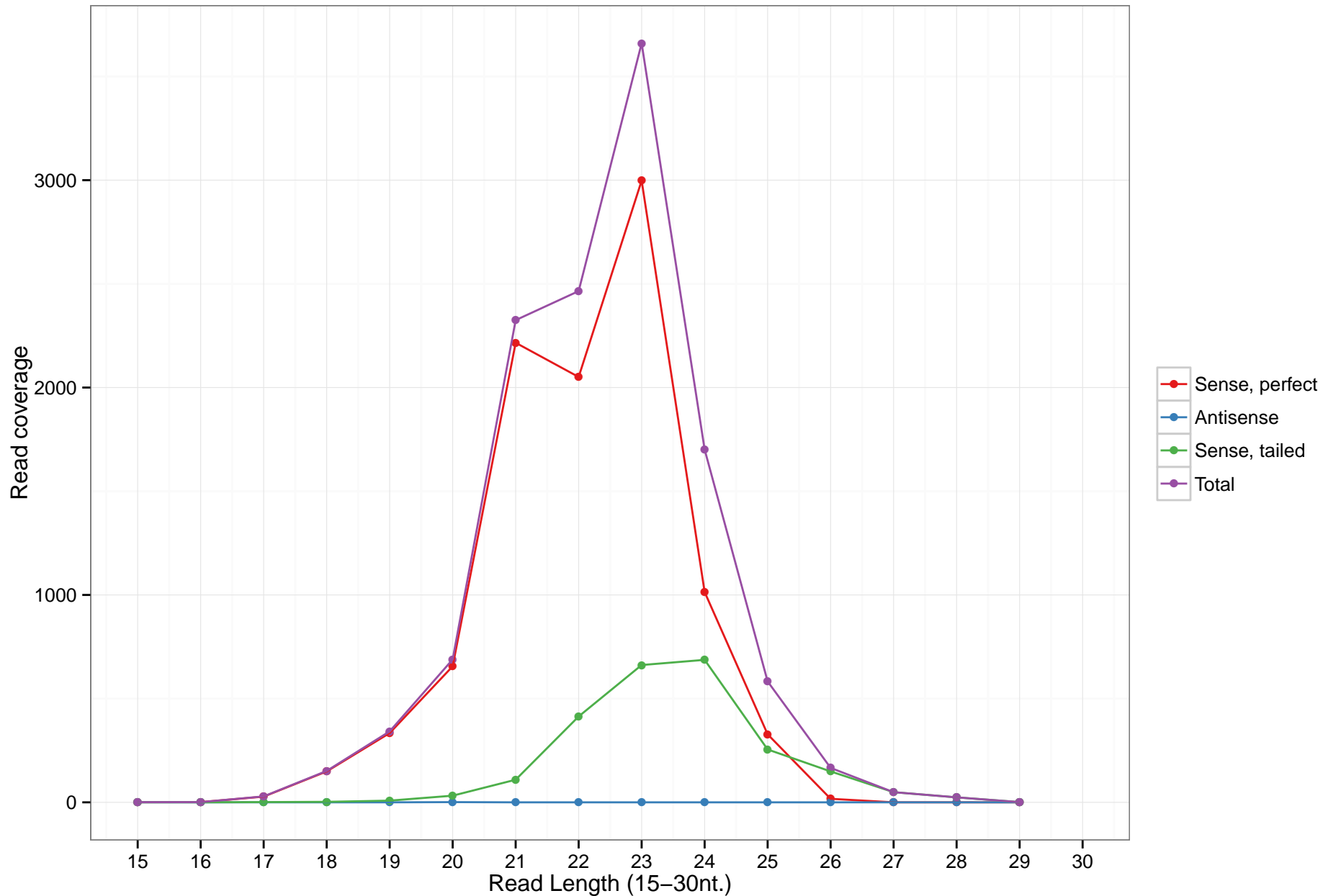
hsa-mir-3605
