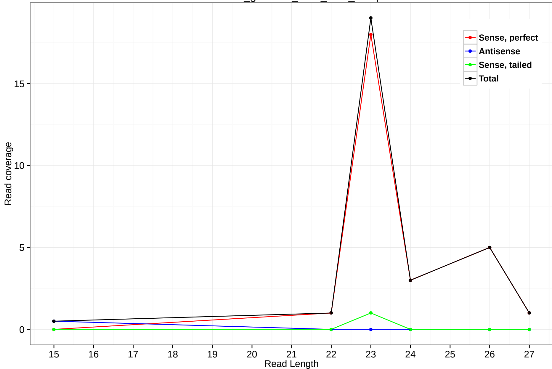
rheMac3_genscan_chrX_61.8_66.3p
