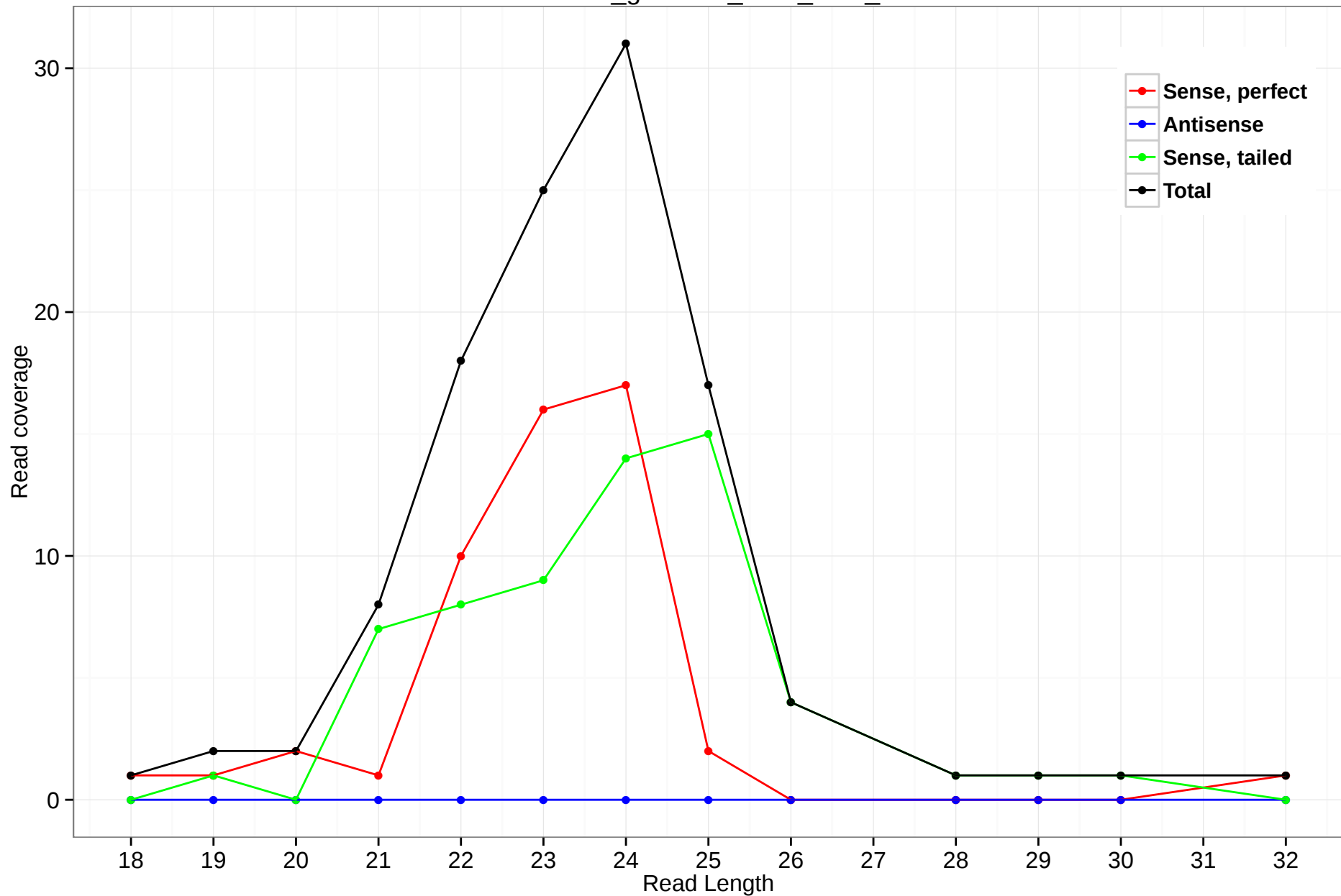
rheMac3_genscan_chrX_61.4_29
