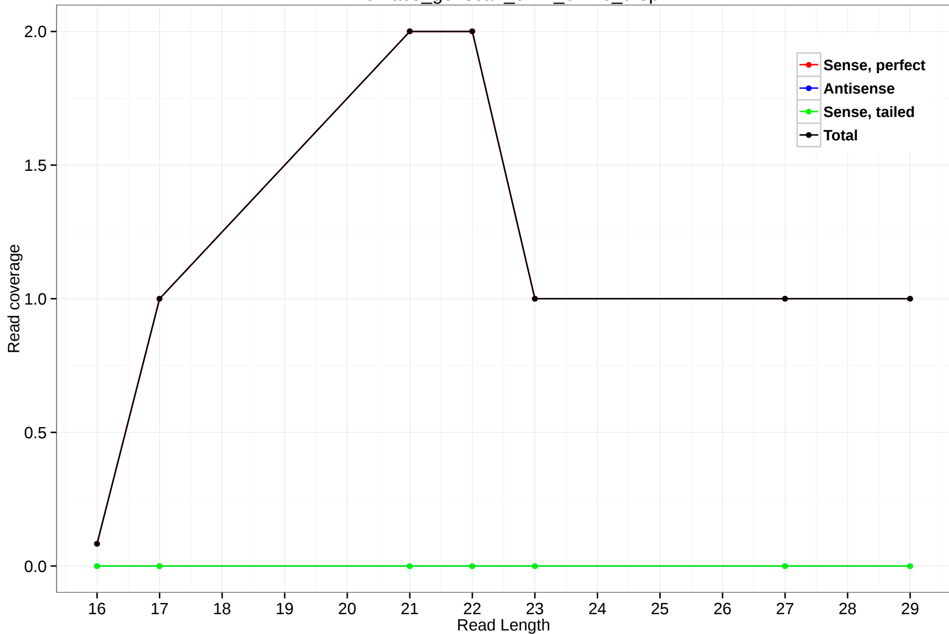
rheMac3_genscan_chrX_61.18_9.3p
