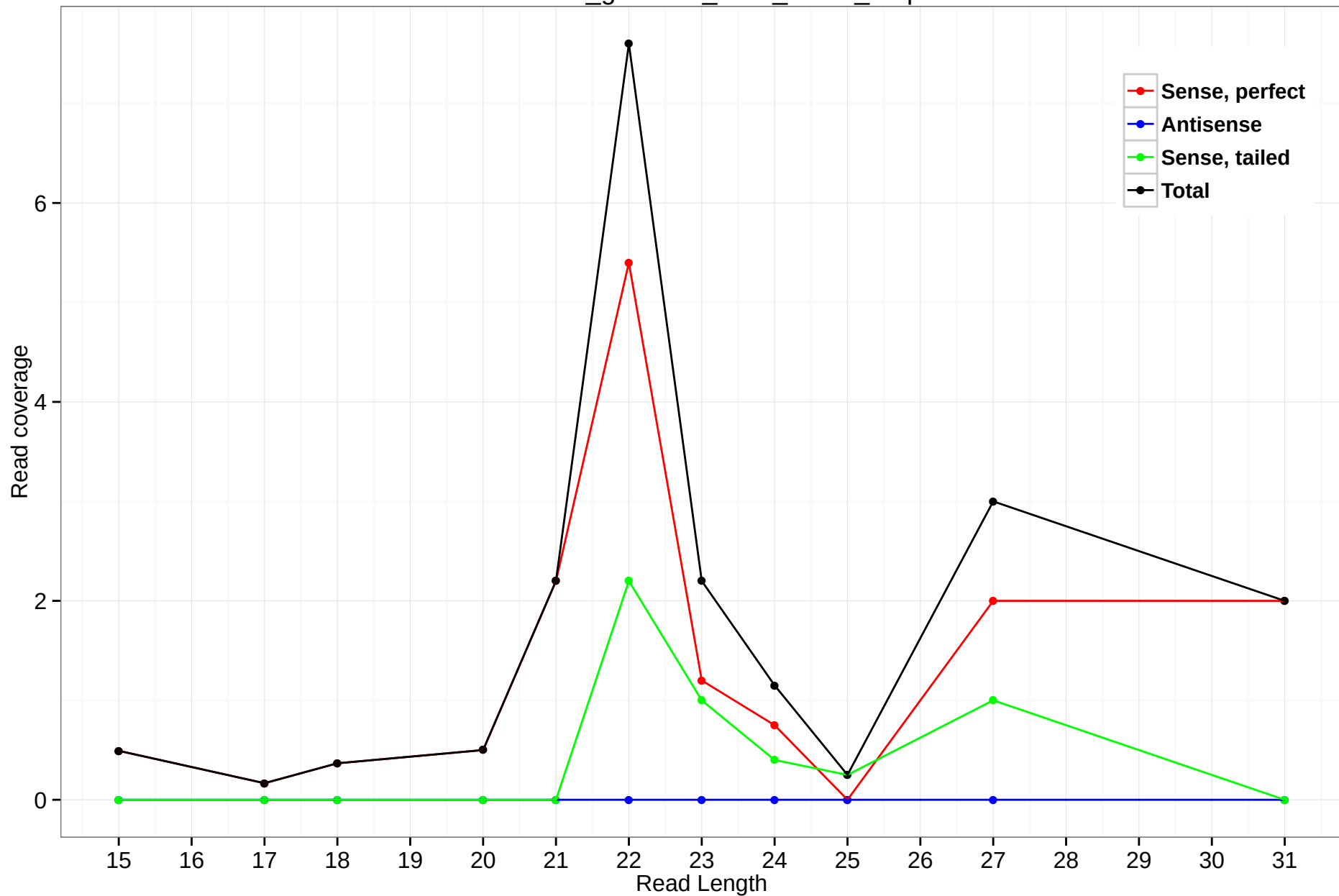
rheMac3_genscan_chrX_61.18_8.3p
