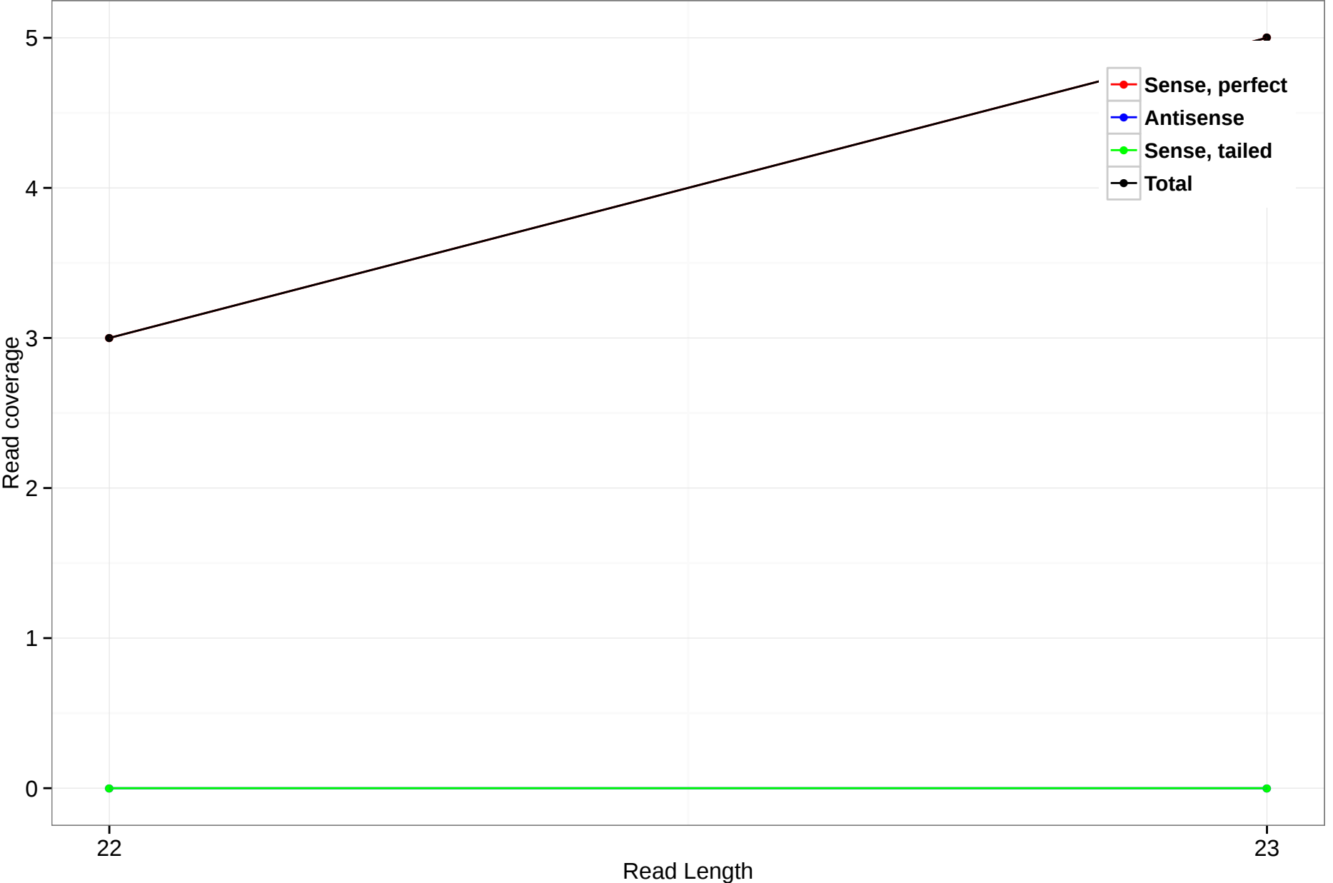
rheMac3_genscan_chrX_40.9_4
