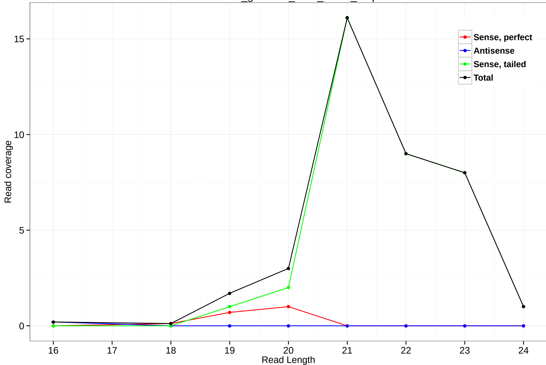
rheMac3_genscan_chrX_34.31_1.5p
