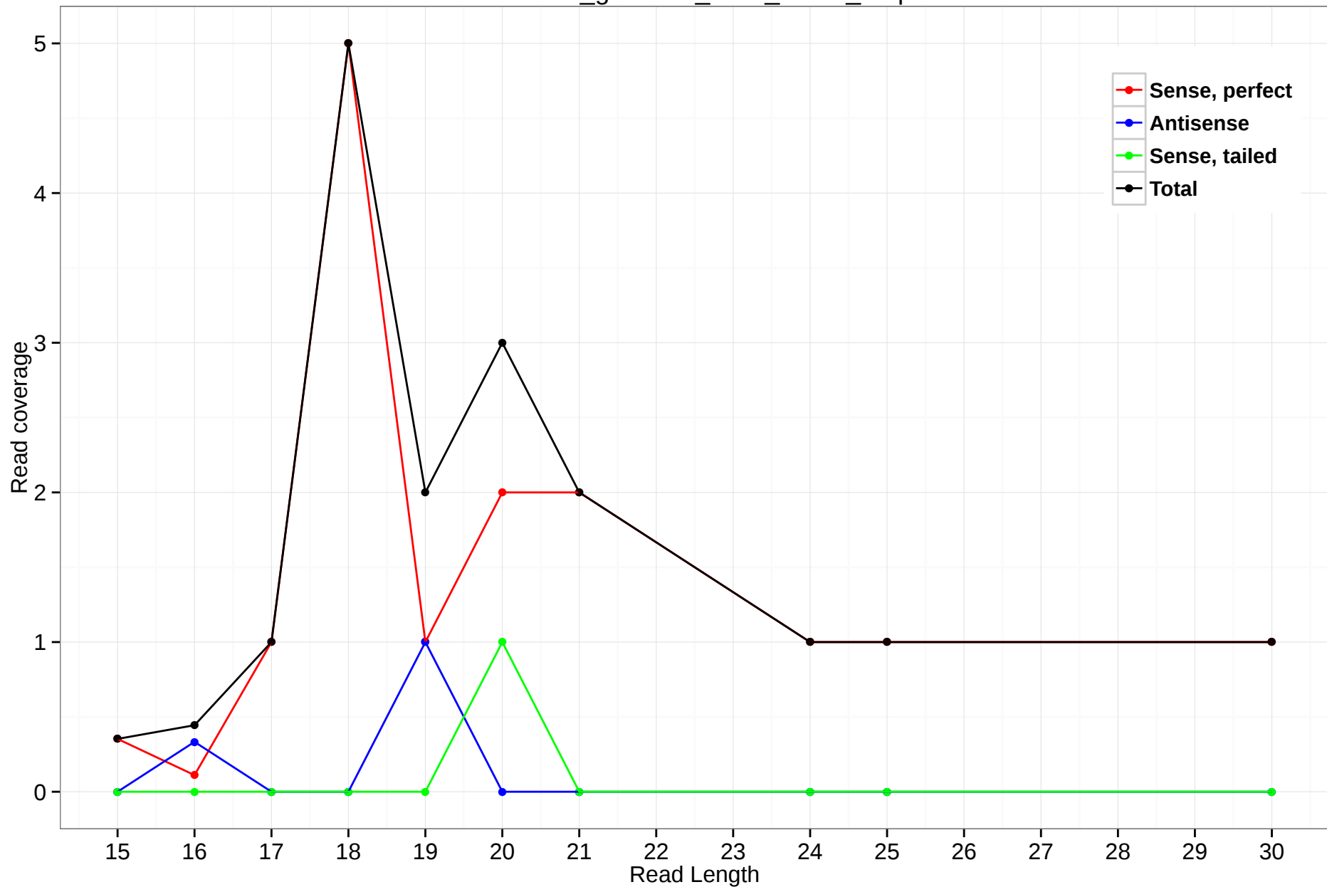
rheMac3_genscan_chrX_34.21_1.5p
