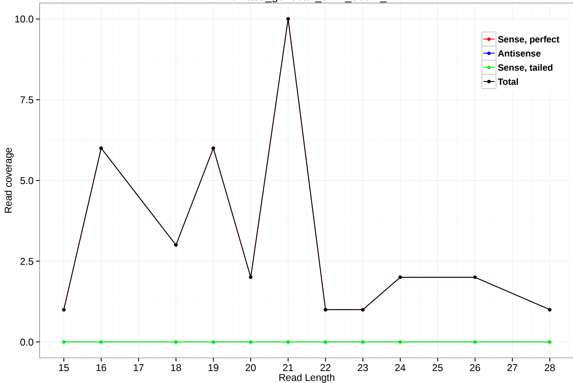
rheMac3_genscan_chrX_306.1_1
