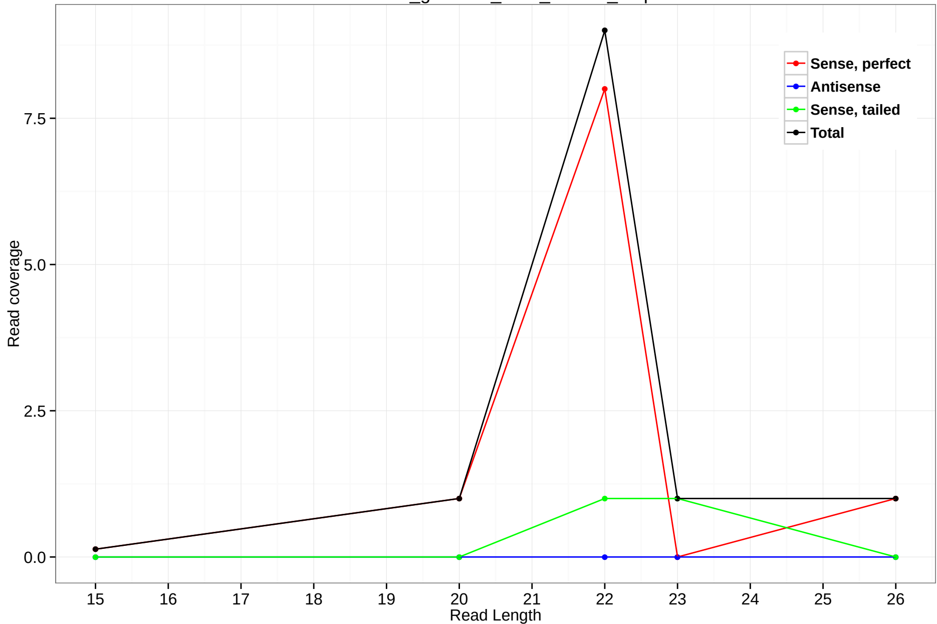
rheMac3_genscan_chrX_306.10_1.3p
