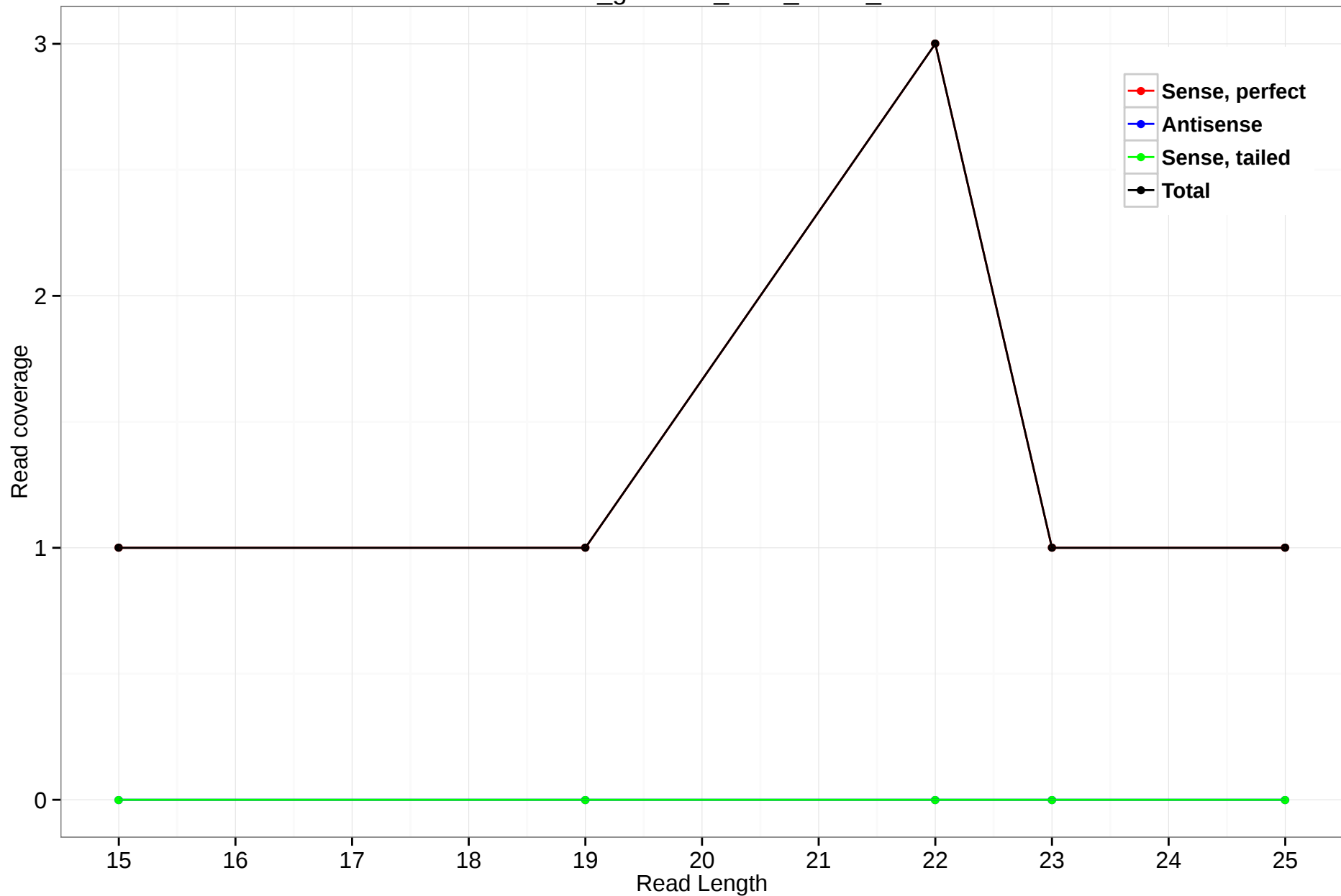
rheMac3_genscan_chrX_305.1_43
