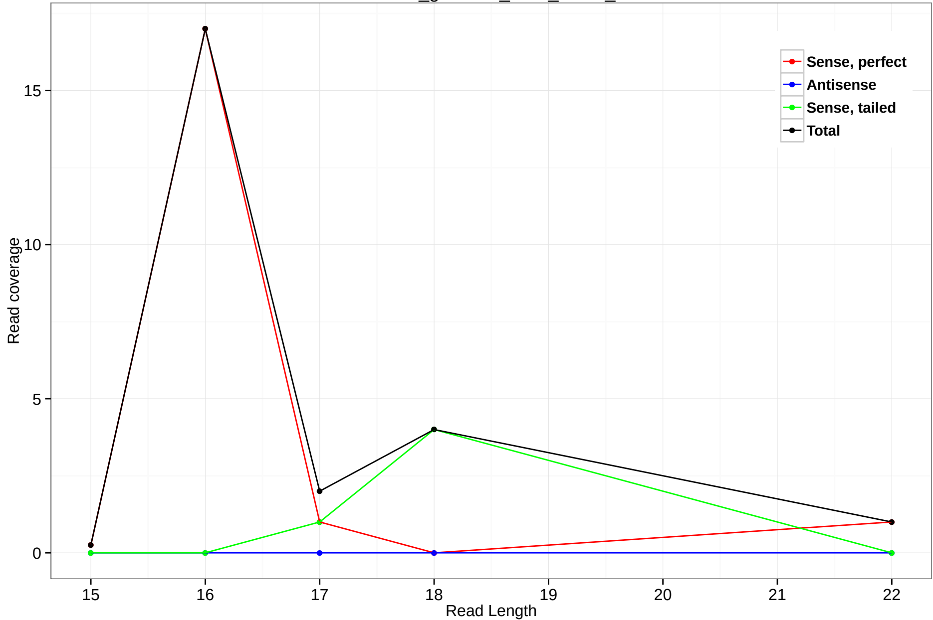
rheMac3_genscan_chrX_305.1_33
