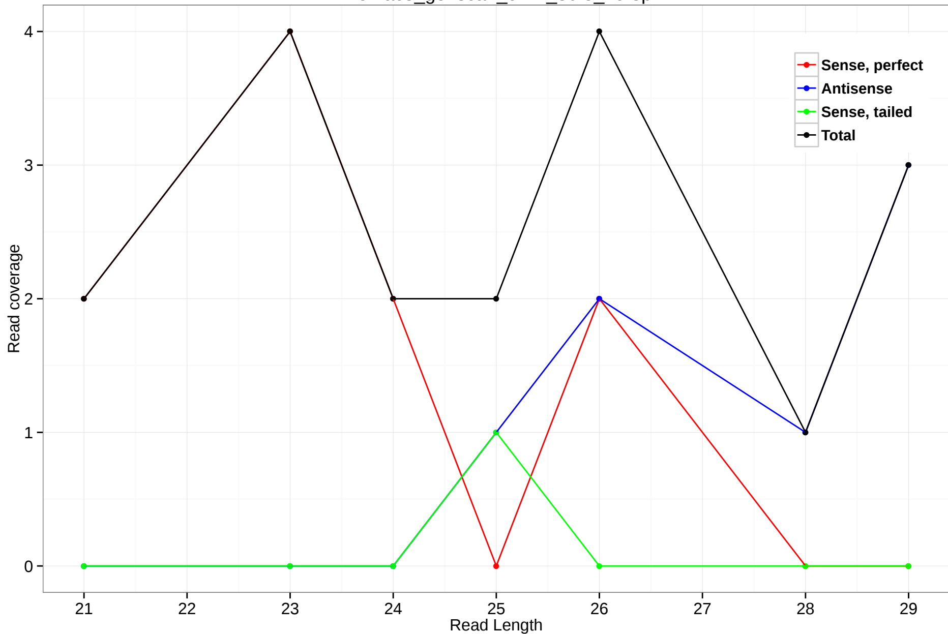
rheMac3_genscan_chrX_30.5_19.3p
