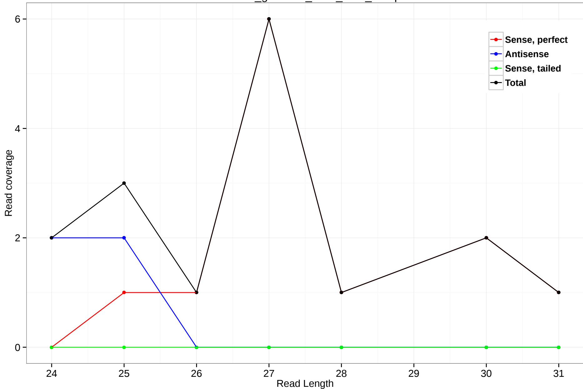
rheMac3_genscan_chrX_30.5_14.3p
