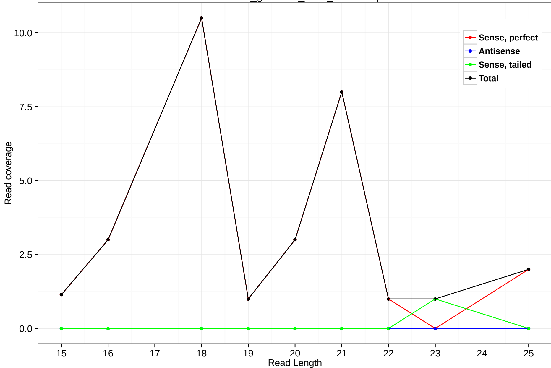
rheMac3_genscan_chrX_298.24.3p
