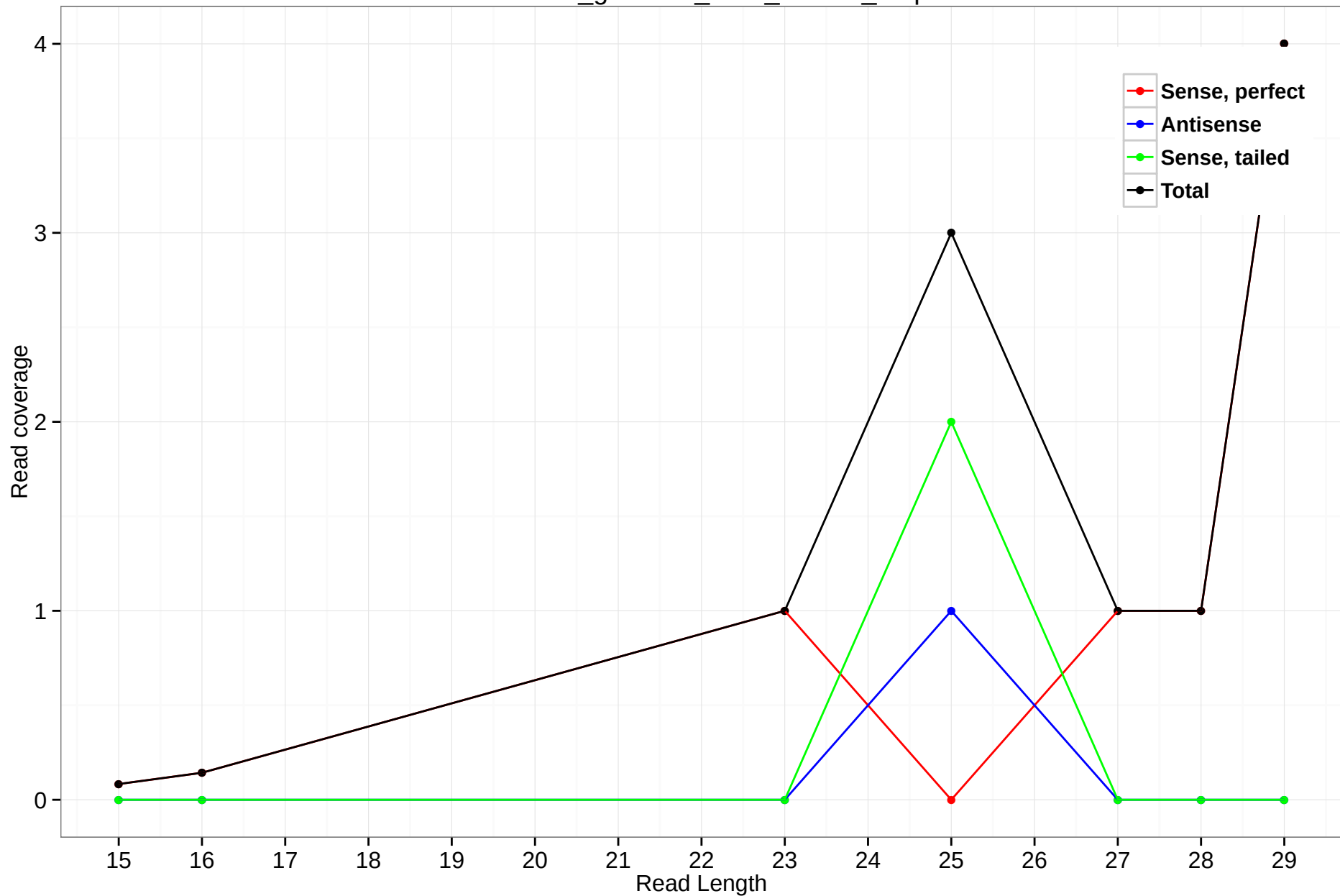
rheMac3_genscan_chrX_298.21_2.5p
