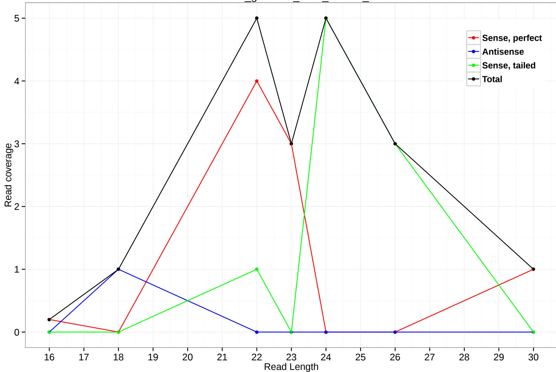
rheMac3_genscan_chrX_298.12_28
